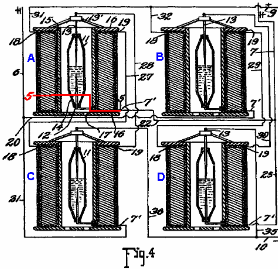
Fig. 4 is a detail view, partly in elevation and partly in section, showing the connections of the converter and intensifier.
