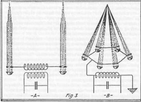
This illustration, from a July 31, 1934 New York Times article, shows several of the special solid aluminum Tesla bulbs which, as Tesla stated in 1940 (see page 27), no longer required vacuum. The current is placed on the beams by means of the ring-shaped electrodes near each bulb, fed with currents from the coils.
